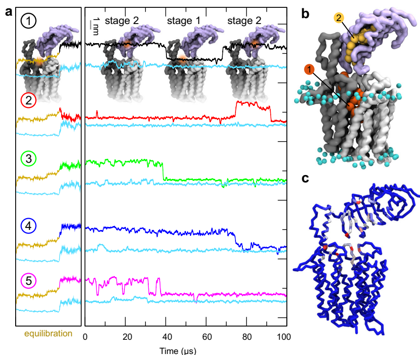
Fig. 6 | TAG transfer into LprG in the MD simulations of the MHAS2168 OUT -LprG complex. a For each of the five simulations (numbered 1–5), the upper line depicts the z-coordinate of the center of mass of the TAG molecule. The cyan lines below correspond to the z-coordinate of the average center of mass of the phosphate groups of the upper membrane leaflet. The gold line is the equilibration phase (see methods). The models of the MHAS2168 OUT -LprG complex shown in the top panel
